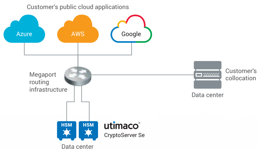
Utimaco CryptoServer Cloud architecture
